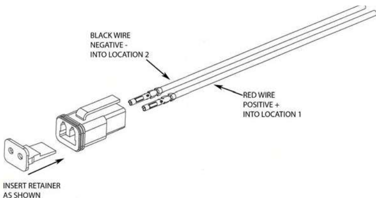
Figure 3 Wiring
