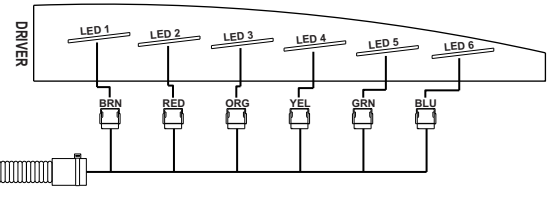
BOTTOM SIDE VIEW
