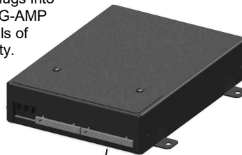
12-Terminal Connector for 8-Output Traffic Director
